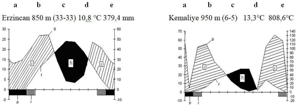
Figure 2. Omrothermic diagrams of Erzincan and Kemaliye (a- station; b- altitude; c-observation period; d- mean temperature; e- annual rainfall).
